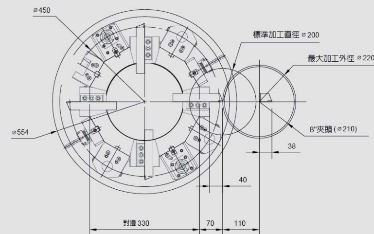
FTC-15MY Tool Interference
